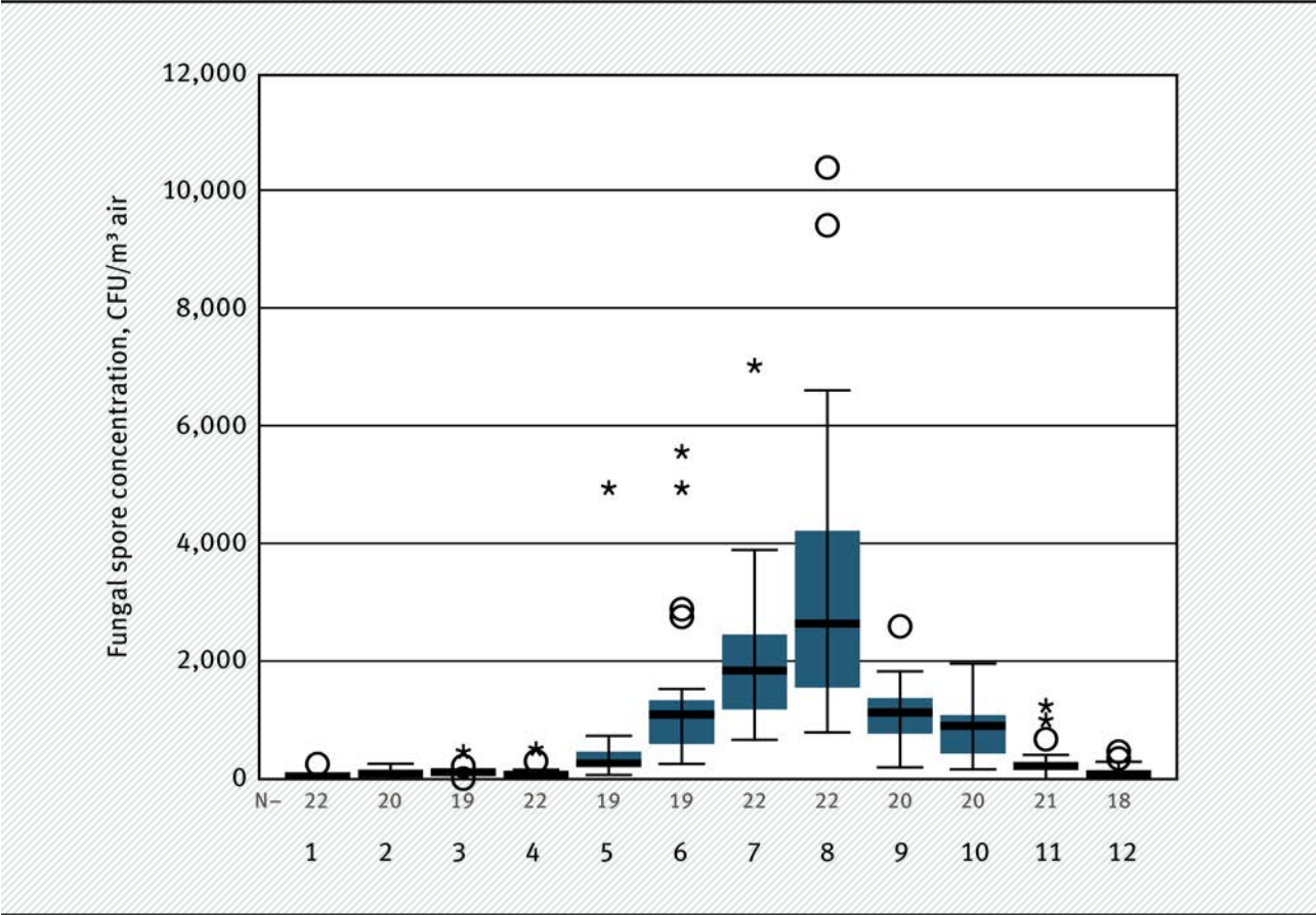
Typical seasonal trend of mould fungus concentration in the outdoor air in Germany
