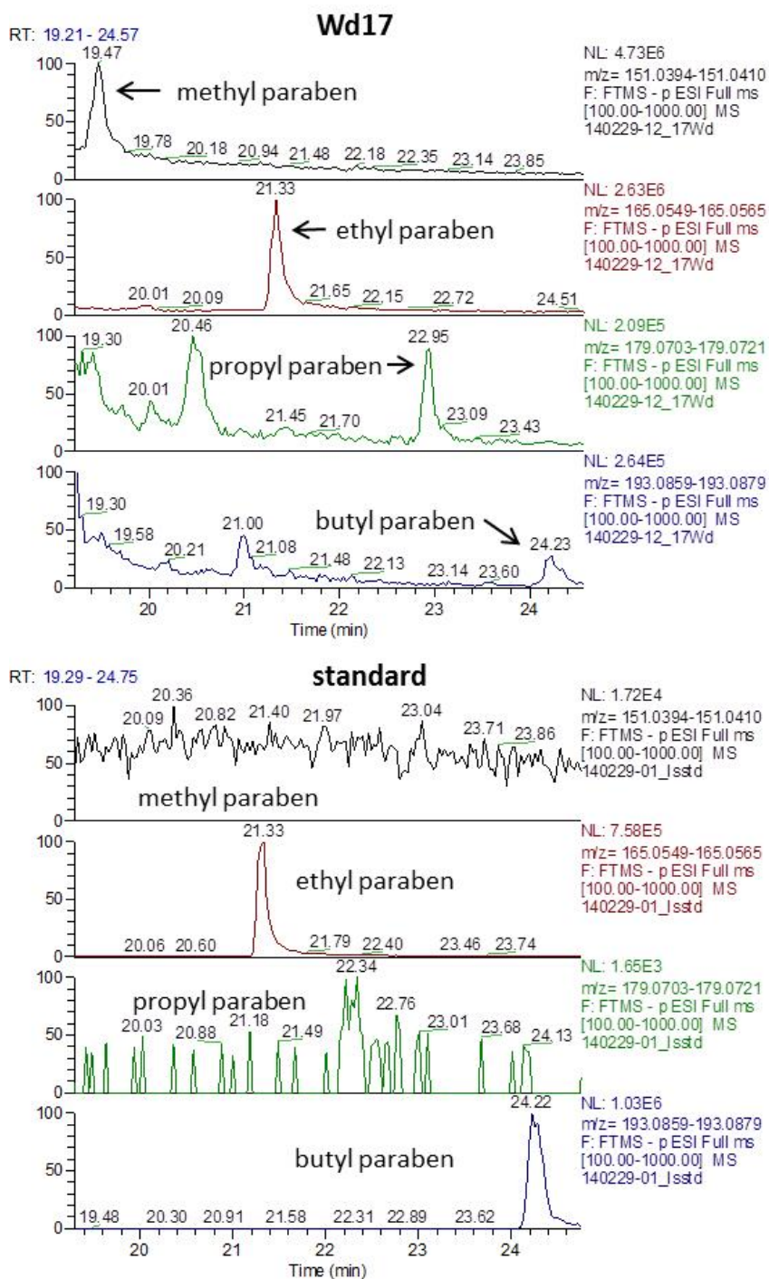
Figure 21: Extracted chromatograms of the four detected parabens (methyl, ethyl, propyl and butyl paraben) in the sample W17 (deconjugated extract) and a standard, showing matching RTs.
