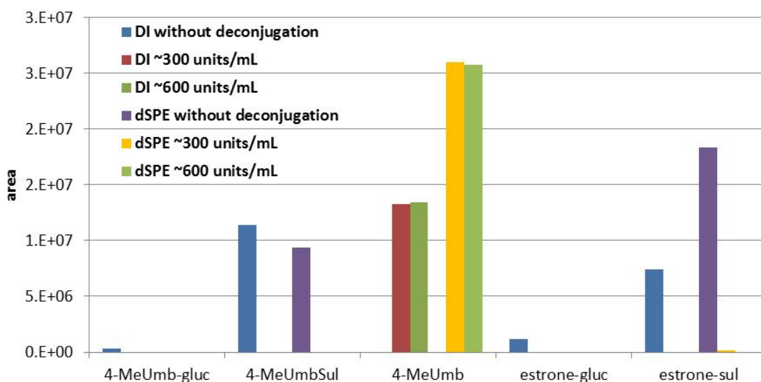
Figure 11: Peak areas for conjugates (4-MeUmb-glucuronide and -sulfate, estrone-glucuronide and sulfate) and the unconjugated 4-MeUmb in samples without and with deconjugation by \beta -glucuronidase.
