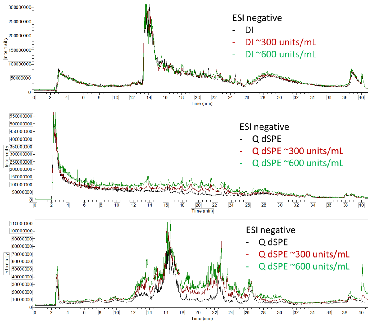
Figure A 1: TICs of DI and QdSPE extracts, comparing the deconjugated and not-deconjugated samples.
