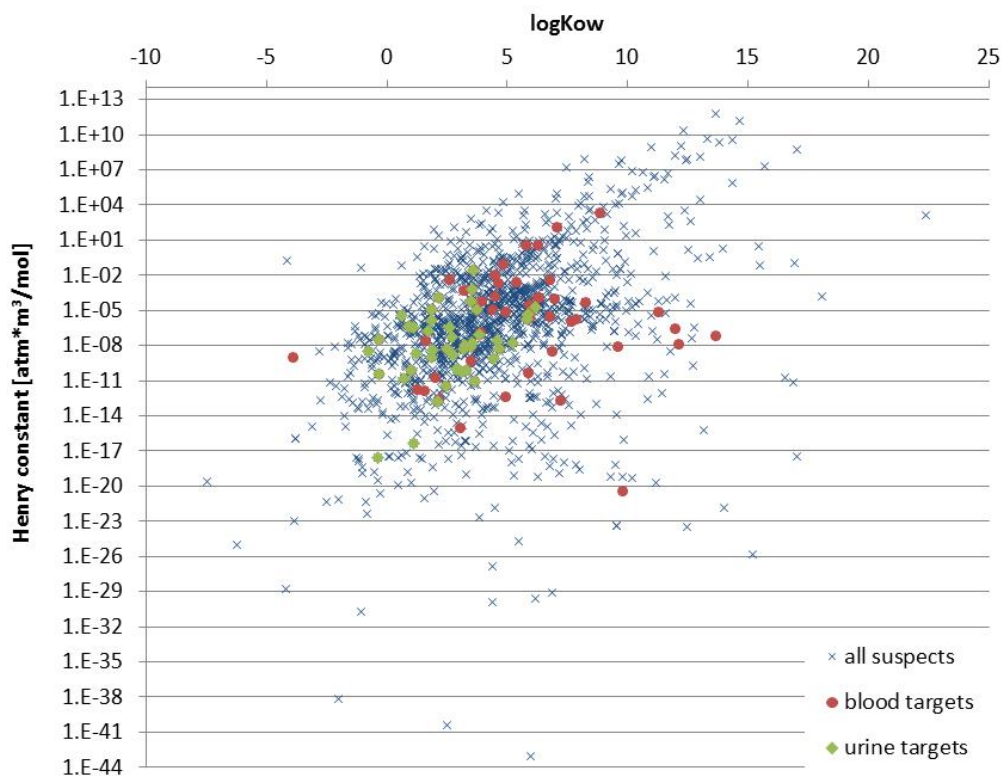
Figure 5: Chemical space plot; distribution of \log K_{ow} and Henry constants of the selected target substances for blood and urine compared to all 1500 suspects.
