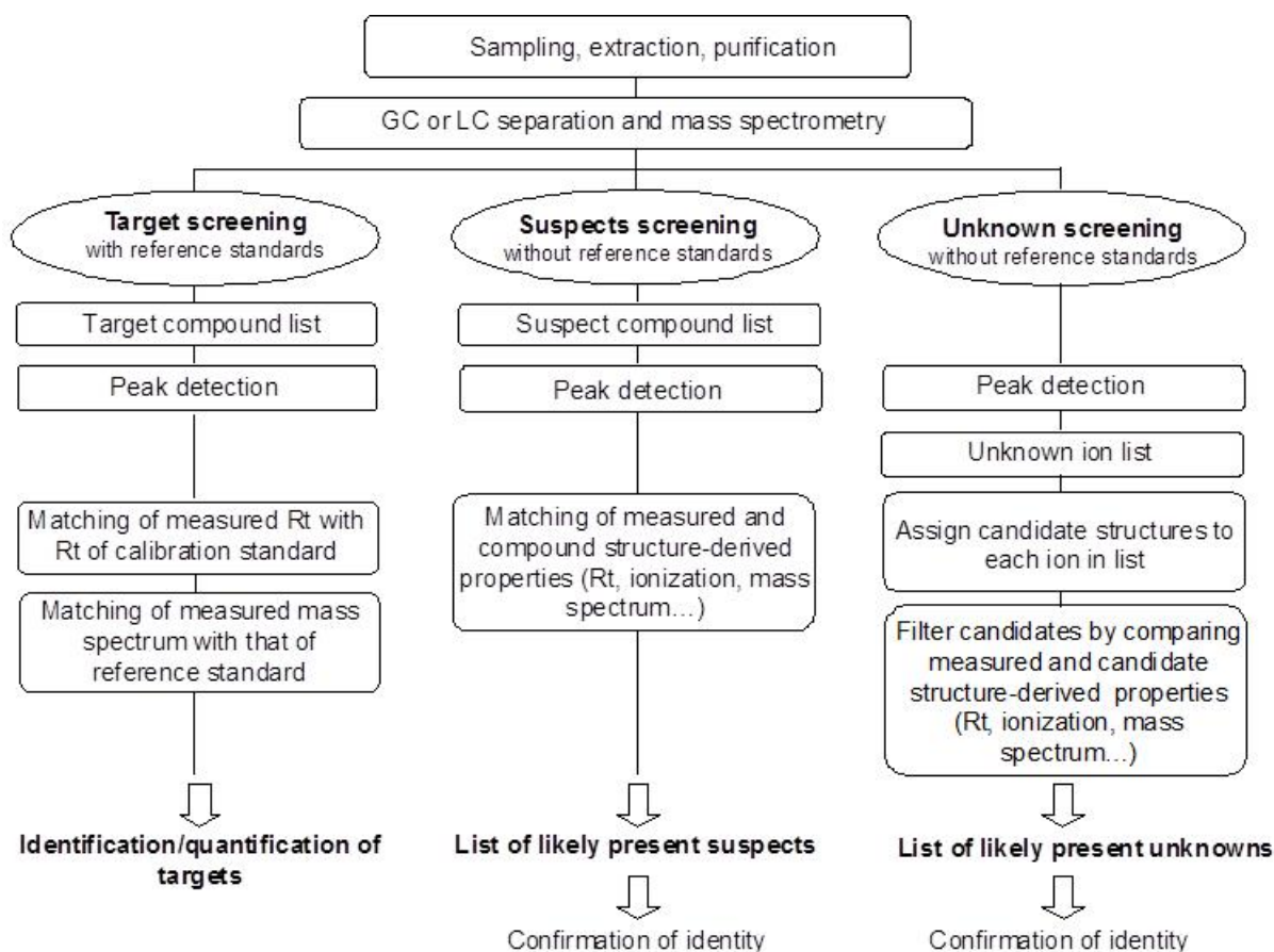
Figure 1: Comparison of systematic workflows for (i) quantitative target analysis with reference standards, (ii) suspect screening without reference standards, and (iii) non-target screening of unknowns in environmental samples by using LC–high resolution (tandem) mass spectrometry. According to [3].
