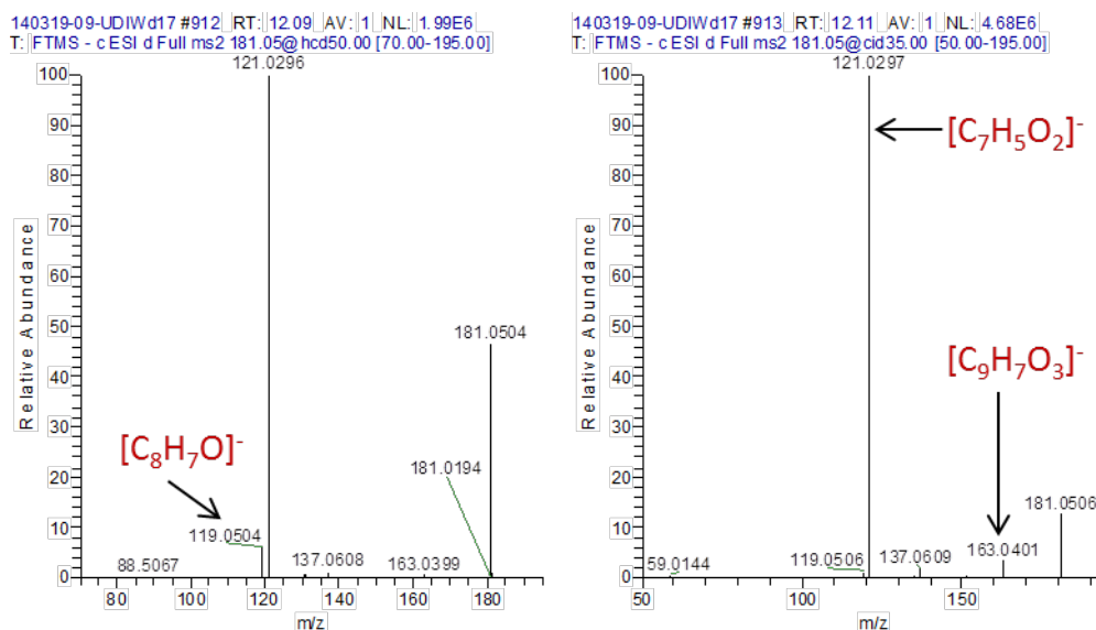
Figure 22: HR-MS/MS spectra of 181.05, left: HCD 50, right: CID 35 with tentatively identified fragment ions for homovanillic acid.
