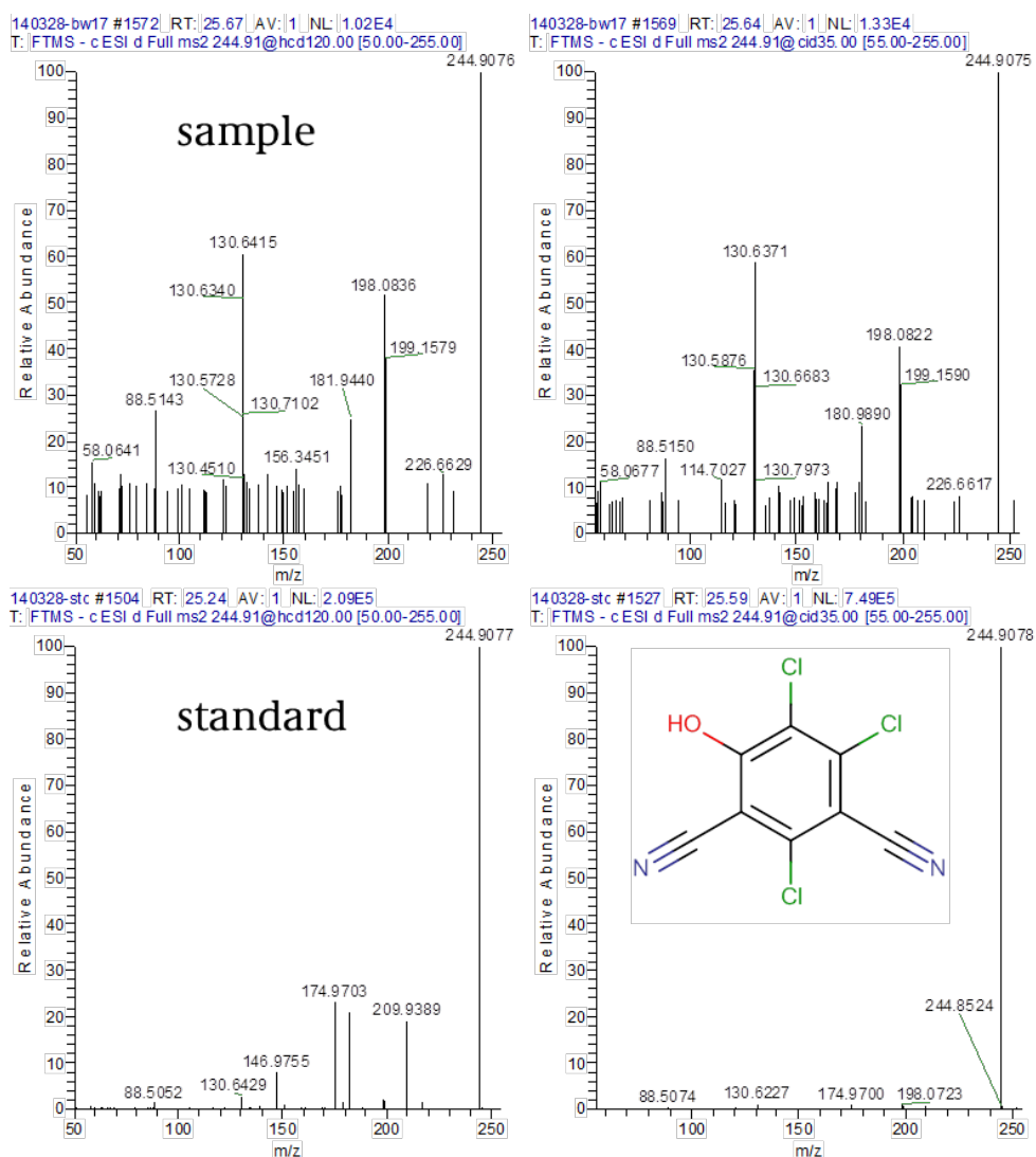
Figure 28: HR-MS/MS spectra of the blood sample W17 (first row) and a reference standard containing 4-hydroxy-chlorothalonil (second row). Left side: HCD 120, right side: CID 35.
