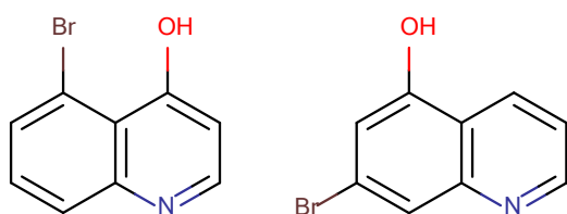
Figure 29: Possible structures of the non-target peak detected with Br isotope pattern.
