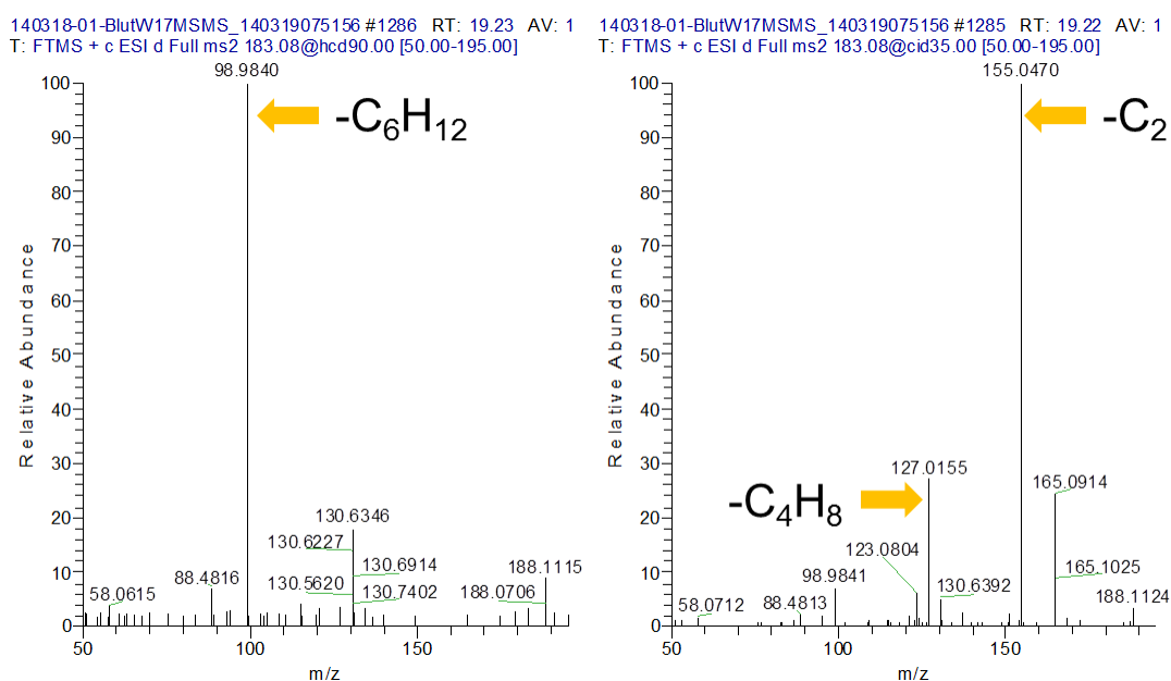
Figure 24: HR-MS/MS spectra of 183.08 in the blood sample W17, tentatively identified as triethylphosphate, left: HCD 90, right: CID 35.
