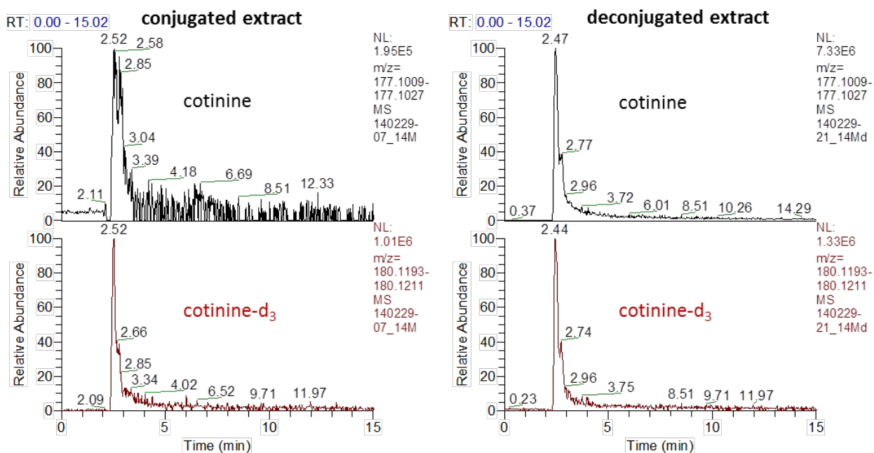
Figure 25: Chromatograms of cotinine and cotinine-d 3 in a urine sample of a smoker, conjugated extract (left) and deconjugated extract (right), showing the same RT of the compound and the IS and lower peak height in the conjugated sample extract.
