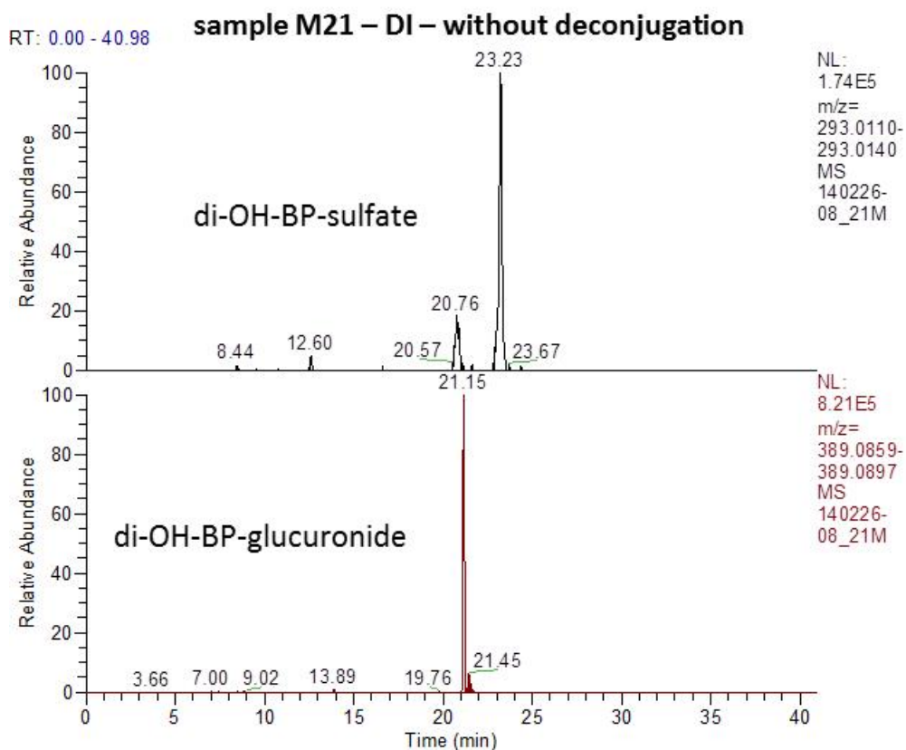
Figure A 3: Extracted ion chromatograms of the calculated m/z values for dihydroxy-benzophenone-sulfate and glucuronide analysed by DI in the still conjugated extract of sample 21.
