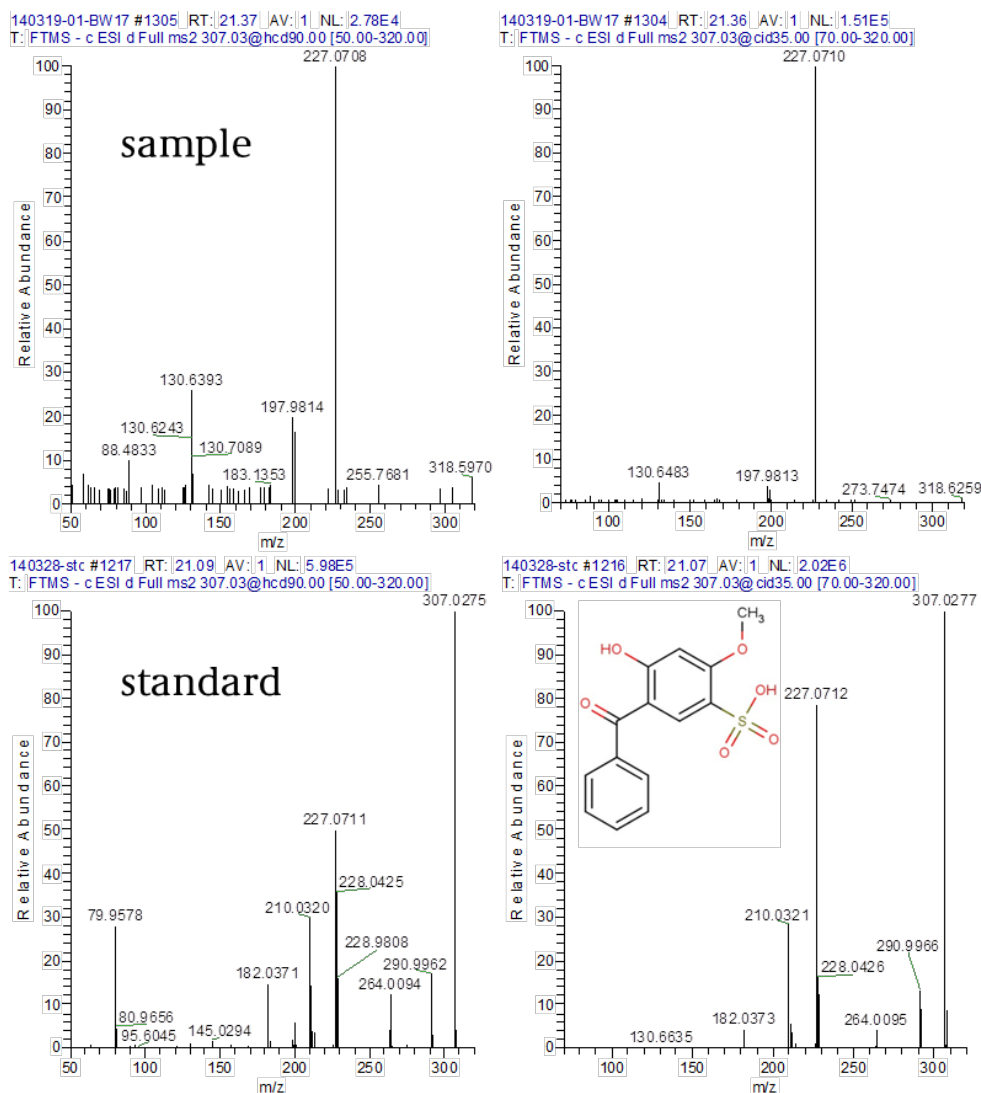
Figure 23: HR-MS/MS spectra of m/z 307.03 in the blood sample W17 (first row) and a reference standard containing benzophenone-4 (second row). Left: HCD 90, right: CID 35.
