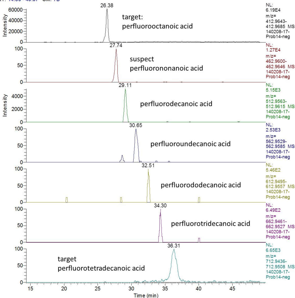
Figure 26: Extracted ion chromatograms of tentatively identified perfluorinated carboxylic acids in sample 14, showing matching RTs of the homologues row of C8 to C14 carbon chain lengths.
