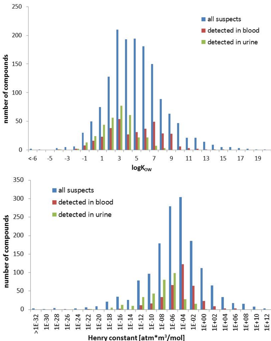
Figure 3: Histograms of \log K_{ow} values and Henry constants ( \text{atm}\cdot\text{m}^3/\text{mol} ) of substances detected in blood, urine and all suspects in the suspect list; predicted using EpiSuite.
