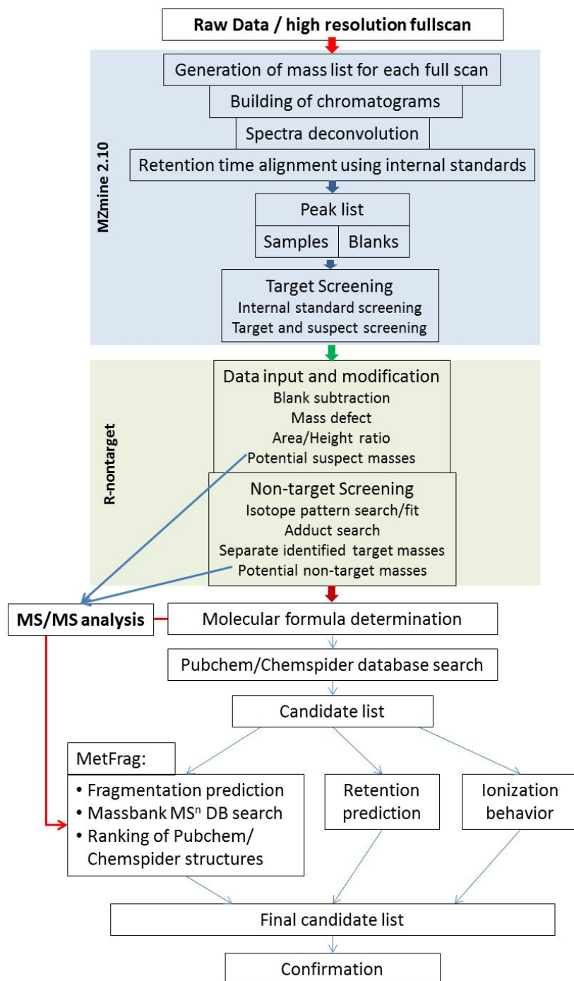
Figure 20: Scheme of data evaluation for LC-MS analysis.
