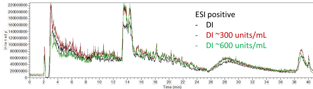
Figure 12: TIC of DI LC-MS analysis in ESI positive mode, comparing the deconjugated and not-deconjugated samples. TICs for negative mode and QuEChERS dSPE extracts can be found in the Annex.
