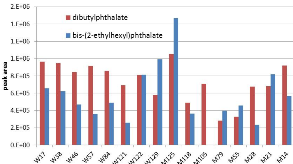
Figure 30: Peak areas of the two detected phthalates in the 16 blood samples.
