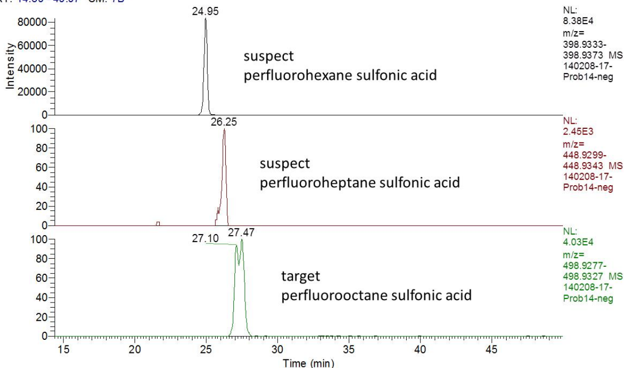
Figure 27: Extracted ion chromatograms of tentatively identified perfluorinated sulfonic acids in sample M14 showing matching RTs of the homologues row of C6 to C8 carbon chain lengths.
