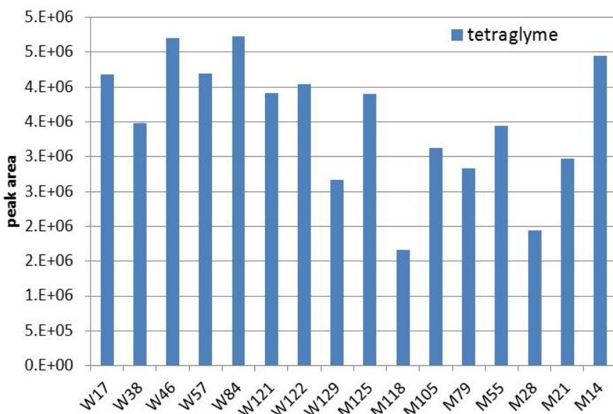
Figure 32: Peak areas of tetraglyme tentatively identified by GC-MS in all blood samples.
