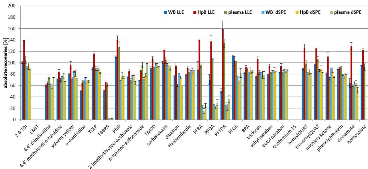
Figure 14: LC-MS analysis: absolute recoveries of target analytes spiked into different blood sample types (50 ng/mL) and extracted by LLE and dSPE: WB - whole blood, HpB - heparin blood, plasma.
