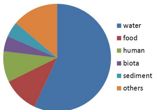
Figure 2: Distribution of sample matrices investigated by the reviewed suspect and non-target screening methods, showing the highest percentage (>50%) for water analysis.
